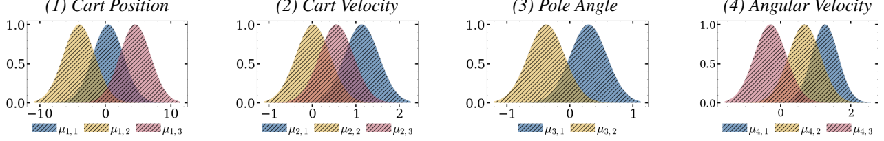
Figure 2: Fuzzy sets found (ordered by moment of creation) when applying CLIP, with \epsilon = 0.6 and \kappa = 0.2 , to Table 1.
