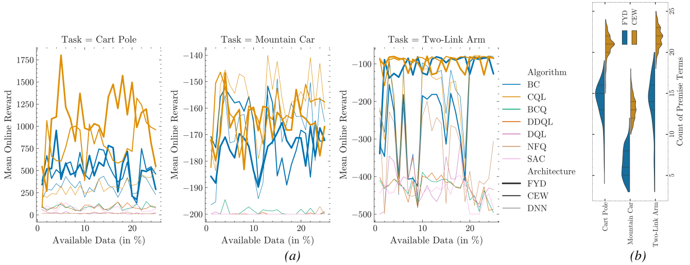
Figure 3: (a) Mean online reward of conditions’ trained policies as more offline data is used; line thickness (determines chosen architecture (e.g., thickest is FYD)). (b) Violin plots show kernel density estimates and quartiles for the premise terms.
